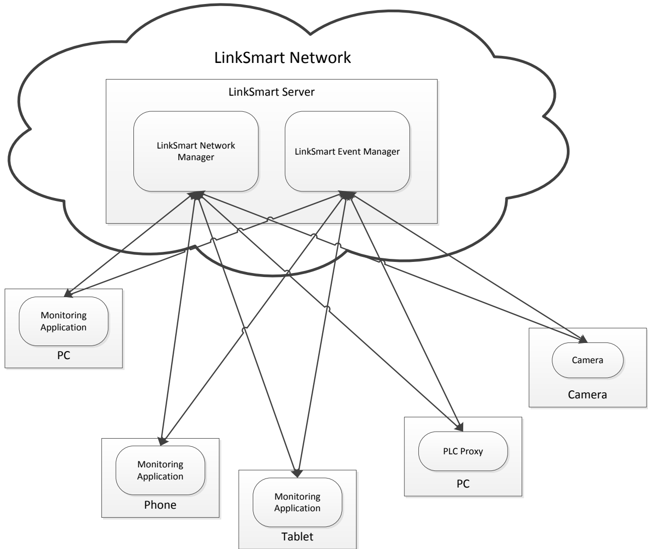
Figure 2: Deployment overview of demonstrator
