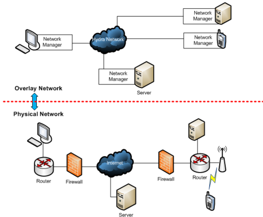
Figure 3: Overlay Network
